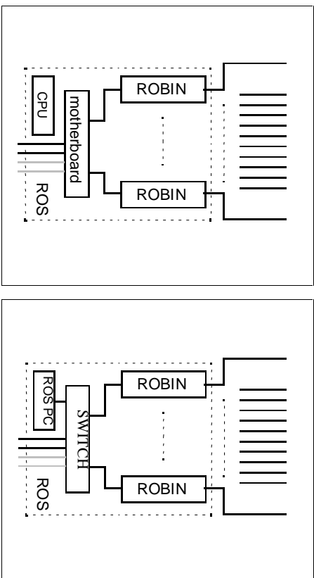
Figure 5-8 The bus based ROS.
