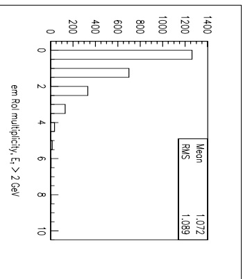
Figure 13-3 EM RoI multiplicity ( E_T > 2 GeV) for events with a muon p_T > 6 GeV.
