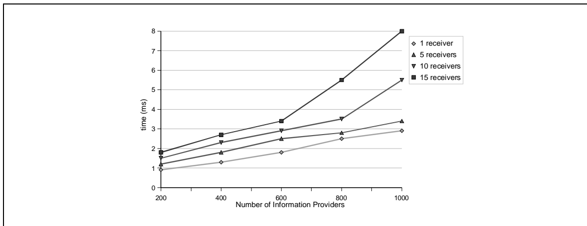
Figure 10-9 Average time spent to transport one information object from one Information Provider to a number of Information Consumers versus the number of concurrent Information Providers
