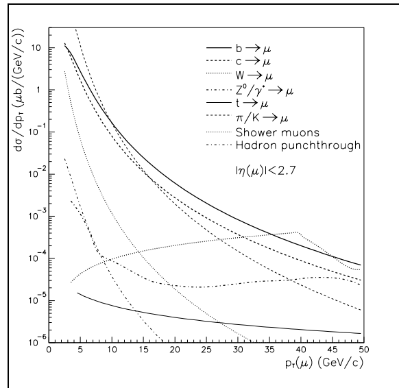
Figure 13-1 Differential cross-section d\sigma/dp_T for inclusive muon production in ATLAS in the pseudo-rapidity range |\eta| < 2.7 .
