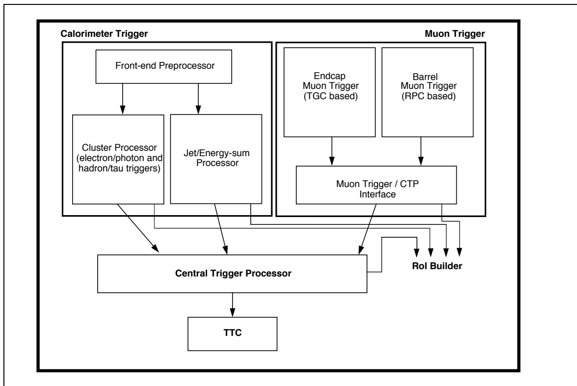
Figure 8-15 [reb001v000_lv11block.eps]
