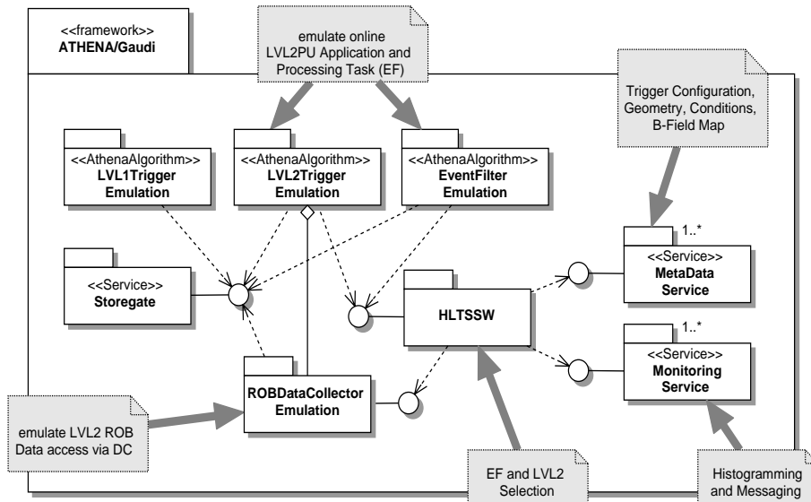
Figure 9-9 (Package diagram showing the dependencies of the event selection software running the LVL2 and EF Selection in the offline. DIAGRAM NEEDS UPDATE! ATHENA IS THE MAIN FRAMEWORK, ROB DATA PROVIDER AND BS CONVERSION SERVICE INSIDE HLTSSW...
