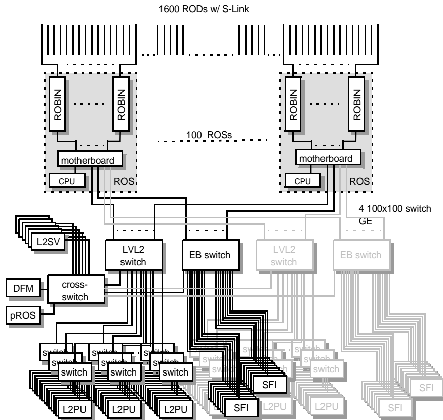
Figure 5-4 Baseline dataflow sketch
