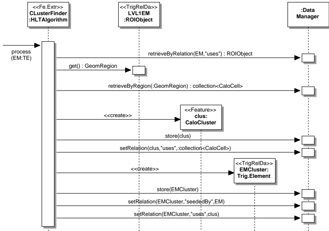
Figure 9-15 Sequence diagram for the cluster finding feature extraction algorithm seeded by an “EM” TE. DIA-GRAM NEEDS UPDATE FOR THE NEW SCHEME OF ACTIVATION OF THE OUTPUT TE, HENCE NAVIGATE BACK TO INPUT TE AND ROI, GET ETA/PHI, RECONSTRUCTION, SAVE CLUSTER AND TRACKS, ACTIVATE TE IF CUT PASSED. - MONIKAS PLOT
