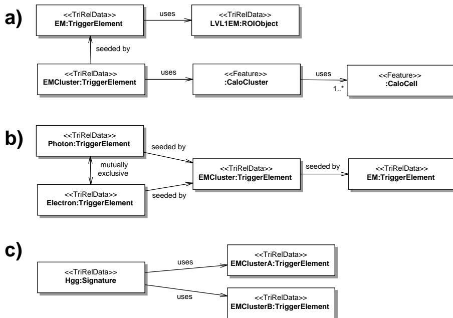
Figure 9-12 Examples of relations between instances of EDM classes, which will be typical for an event processed by LVL2.
