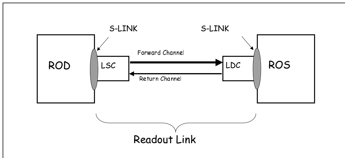
Figure 8-1 The relationship between the S-LINK and the ROL.
