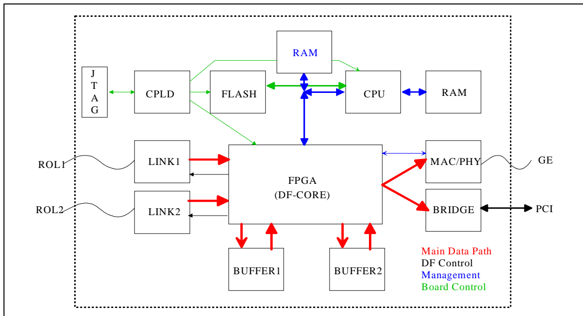
Figure 8-4 Basic Functional Diagram.
