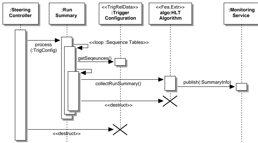
Figure 9-23 A sequence diagram for the Run Summary, which is executed at the end of a “RUN”. CRISTOBAL MAY UPDATE THE DIAGRAM
