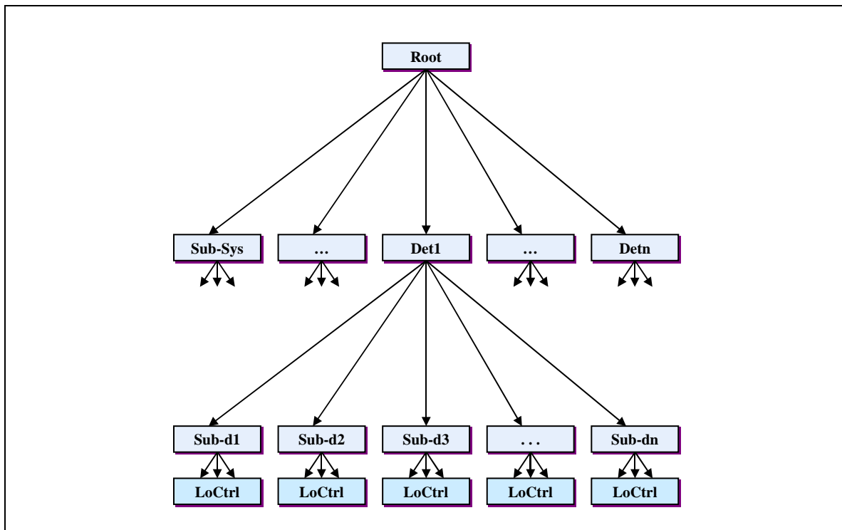
Figure 12-2 Online Software Control Hierarchy in TDAQ
