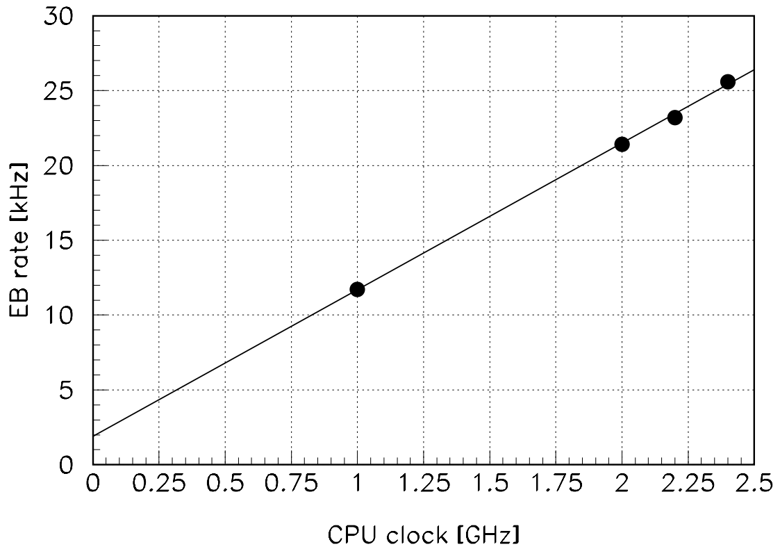
Figure 8-21 Event Building 2.
