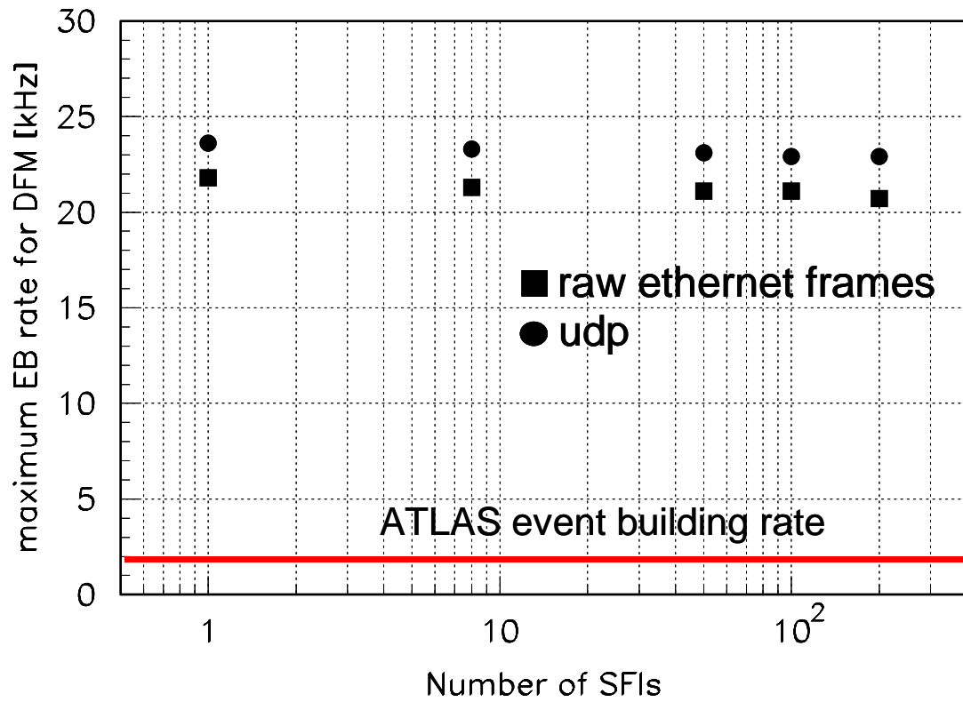
Figure 8-20 Event Building 1.
