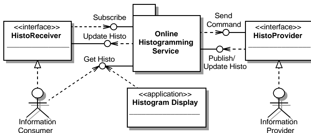
Figure 10-15 Online Histogramming Service interfaces
