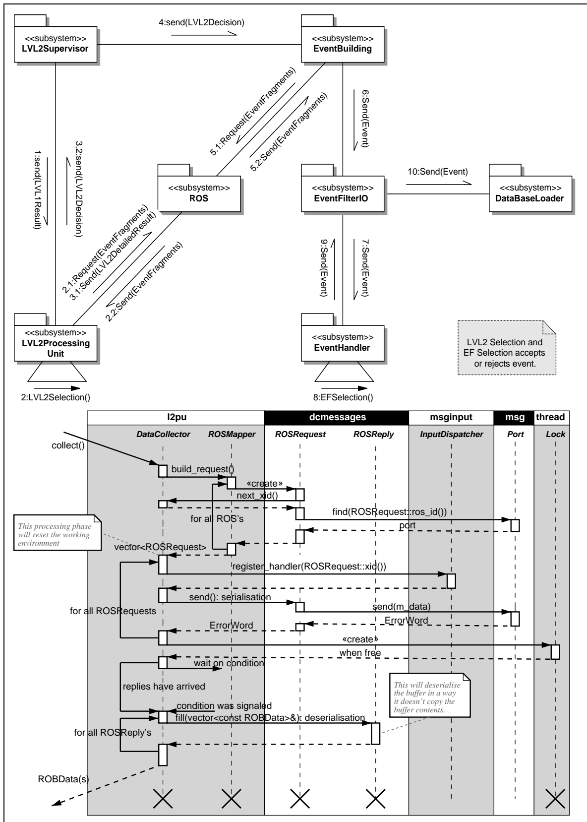
Figure 9-2 Data Collection. Provisional! The two diagrams need to be merged into a simpler (collaboration?) diagram with less technical detail.
