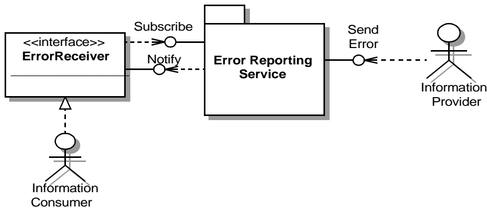
Figure 10-14 Error Reporting Service interfaces
