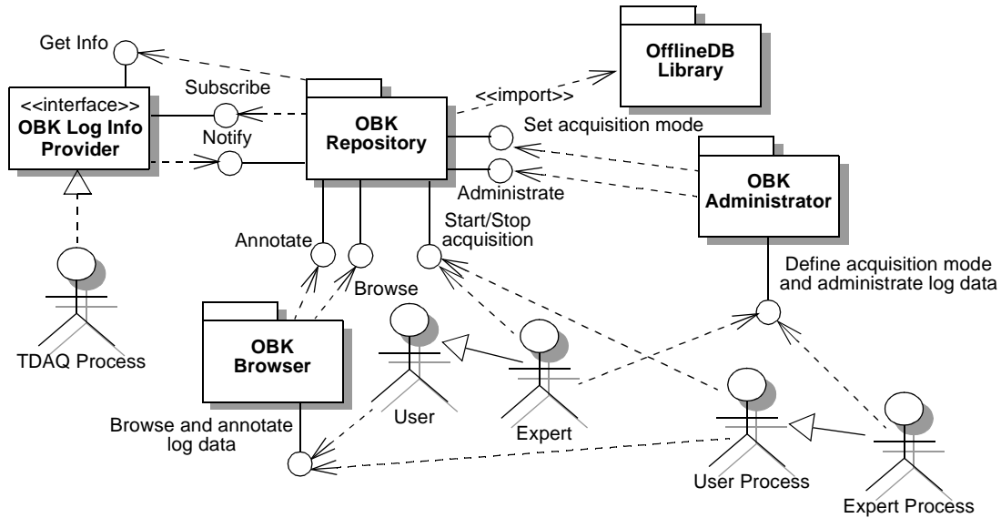
Figure 10-9 OBK users and interfaces
