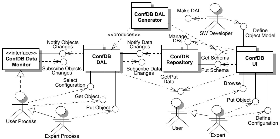
Figure 10-8 Configuration databases users and interfaces
