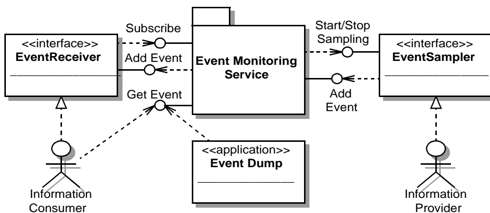
Figure 10-16 Event Monitoring Service interfaces
