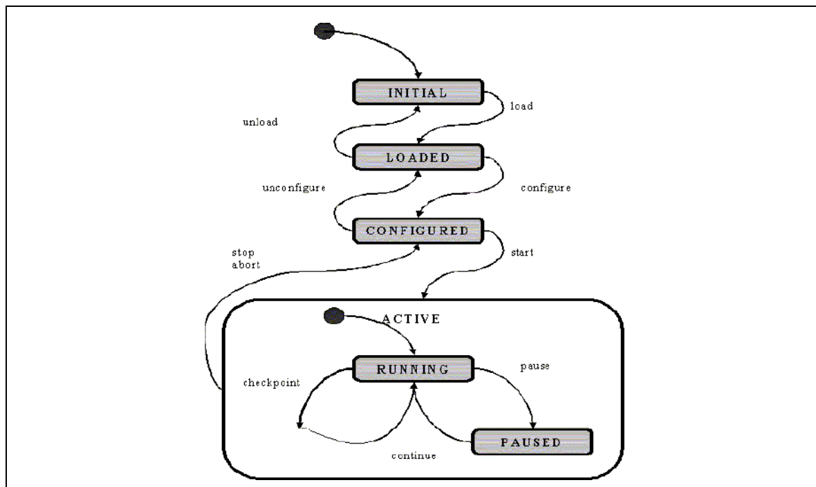
Figure 12-1 TDAQ states
