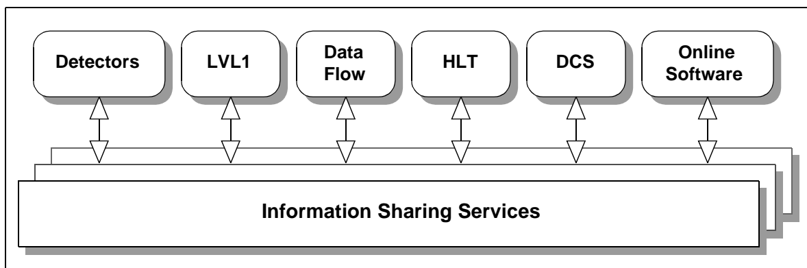
Figure 5-2 Information Sharing context diagram
