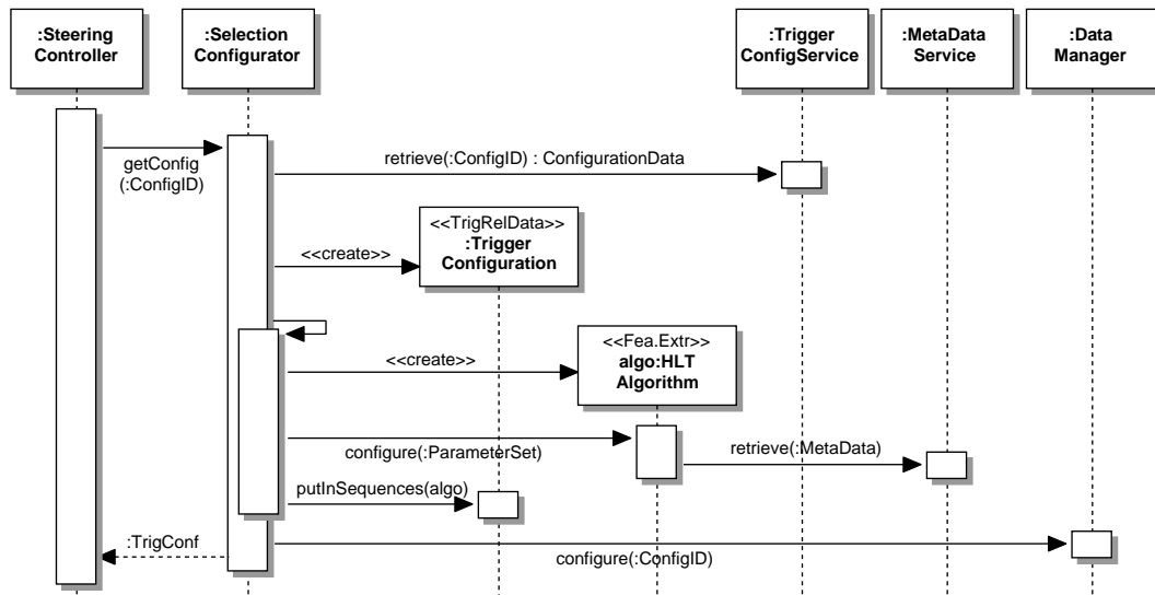
Figure 9-19 A sequence diagram for the Selection Configurator that provides the Trigger Configuration. THOMAS TO UPDATE THIS DIAGRAM.
