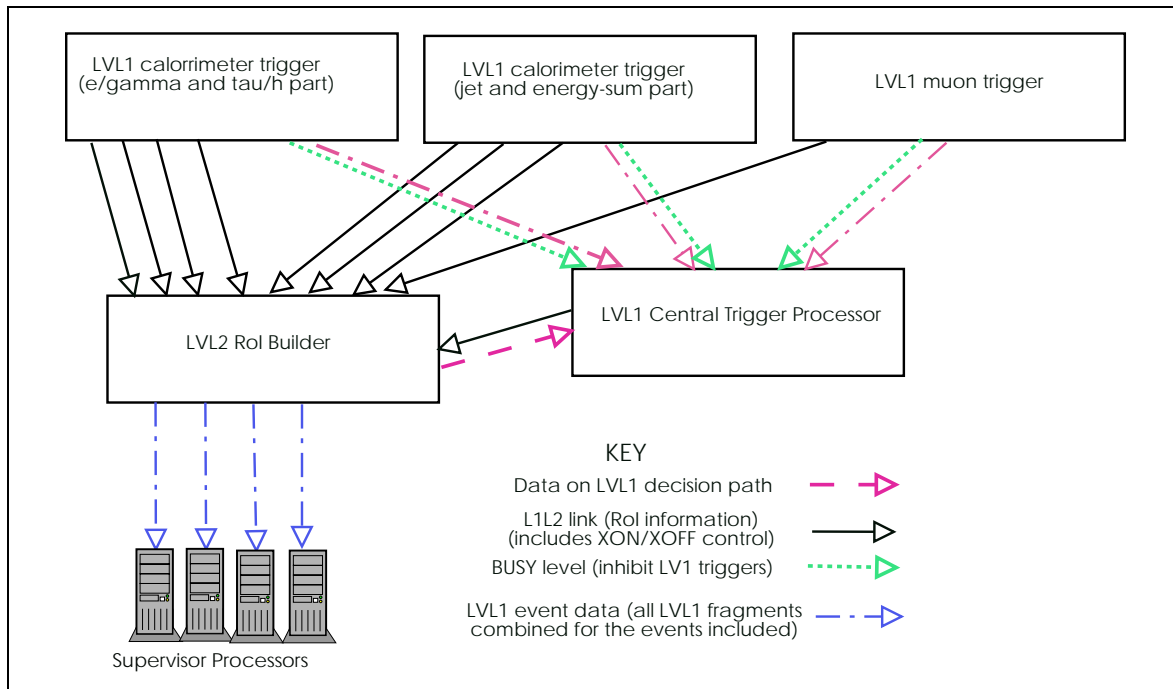
Figure 8-14 [reb001v000_lv11vl2.eps]
