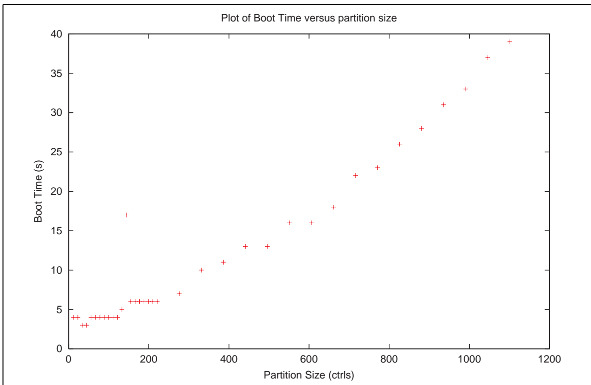
Figure 10-7 Boot transition in a three level control hierarchy for configurations containing 10 to 1000 leaf controllers. To initialize a system with thousand controllers currently 30 seconds are needed.
