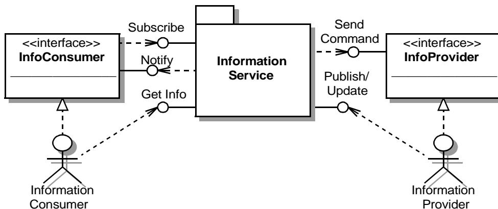
Figure 10-13 Information Service interfaces
