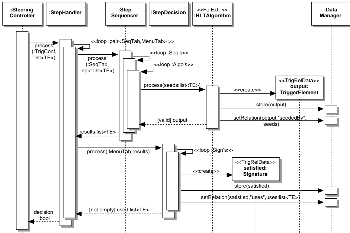
Figure 9-21 A sequence diagram for the step processing showing the role of the step handler, of the sequencer and of the step decision. UPDATE DIAGRAM FOR THE TE ACTIVATION SCHEME -MONIKA.
