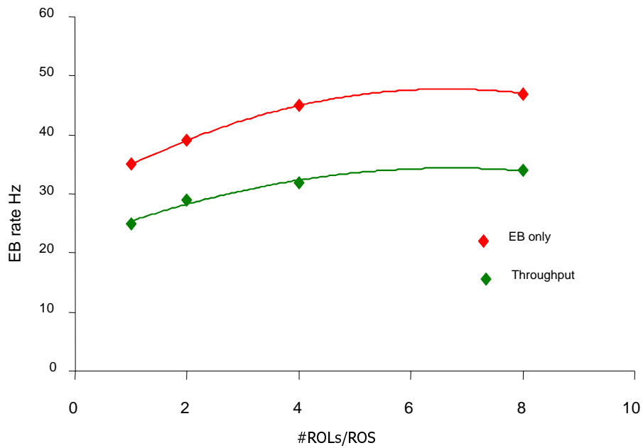
Figure 8-22 Event Building 3.
