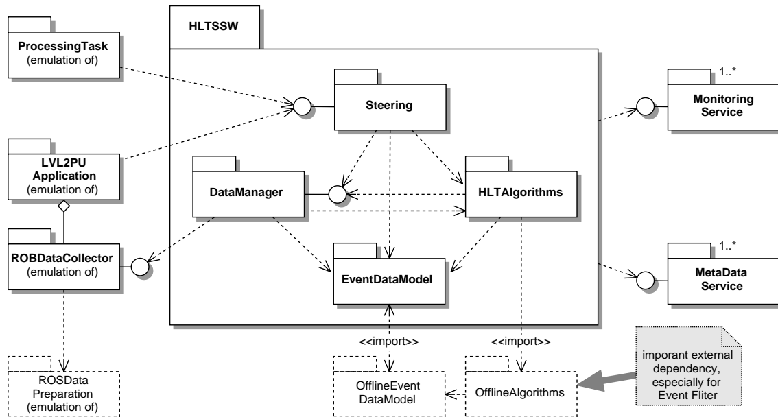
Figure 9-10 A package diagram of the event selection software, showing the dependencies of the sub-packages. The external packages are named following the online case and include their respective offline emulations. The dependencies on the offline event data model and on the offline algorithms are explained in the text. DIAGRAM NEEDS UPDATE, EMULATIONS, DATA MANAGER, PROCESSING TASK-ATHENA EVENT LOOP MANAGER, LV2PU-PSC...
