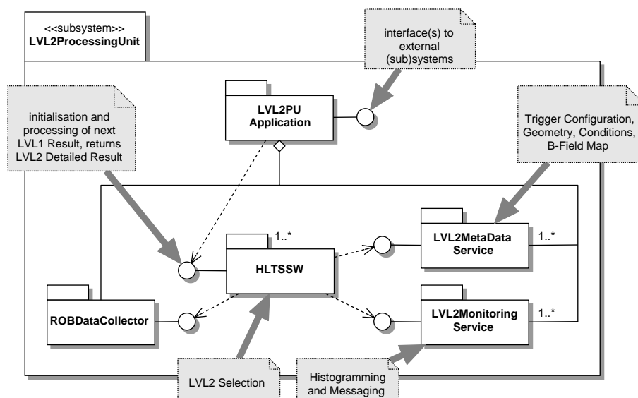
Figure 9-7 Package diagram showing the dependencies of the event selection software performing the LVL2 selection in the LVL2 processing unit. DIAGRAM NEEDS UPDATE (HLTSSW-ESS, PSC,...)
