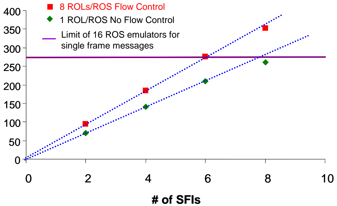
Figure 8-23 8 ROLs/ROS 4.
